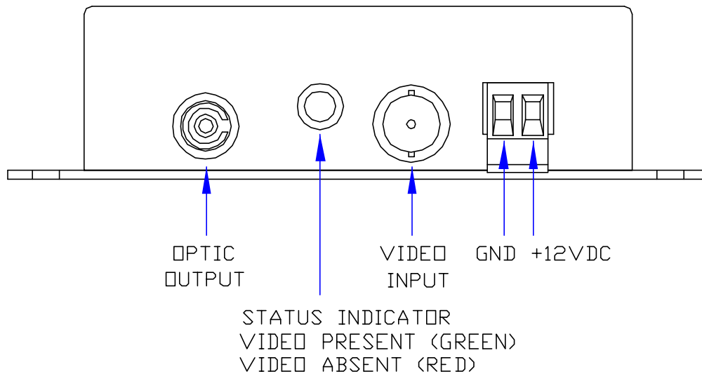
PT-100ME2-X PINOUT DIAGRAM
