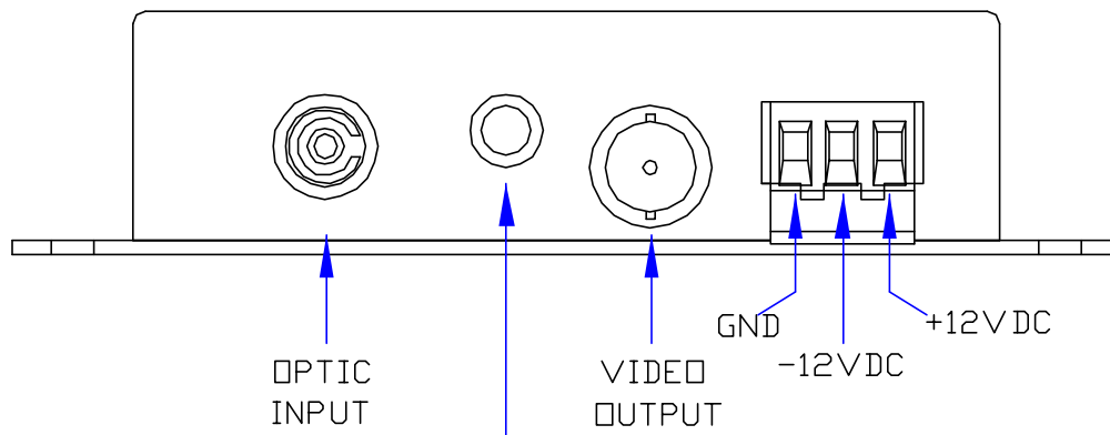
PR-100ME2-X PINOUT DIAGRAM
