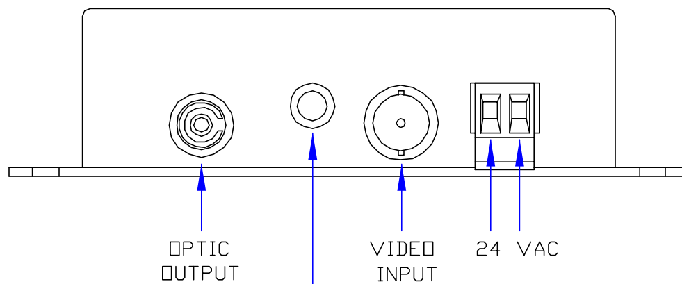
PT140/145M-X PINOUT DIAGRAM
