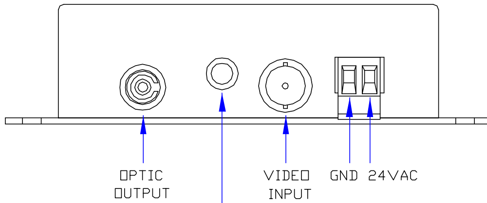
PT-100M-X PINOUT DIAGRAM
