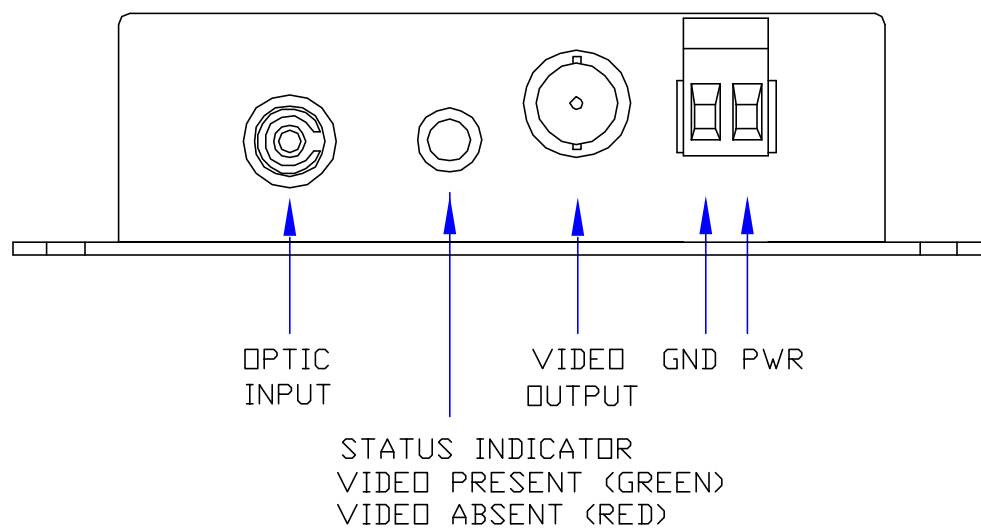
PR-100E-X PINOUT DIAGRAM
