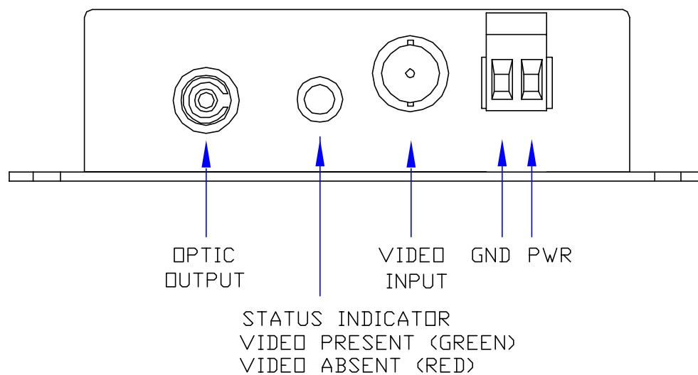
PT-100E-X PINOUT DIAGRAM
