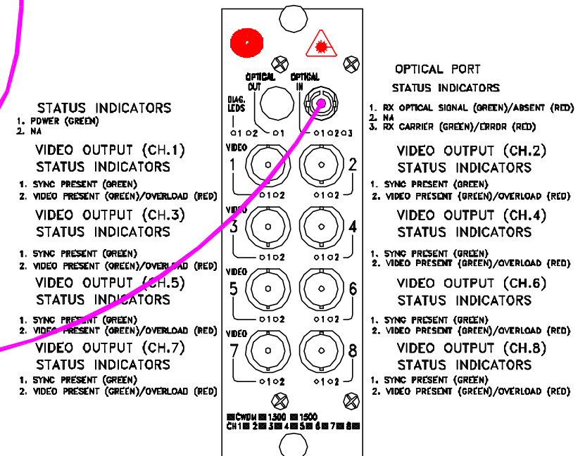
DR-8V-X PINOUT DIAGRAM
