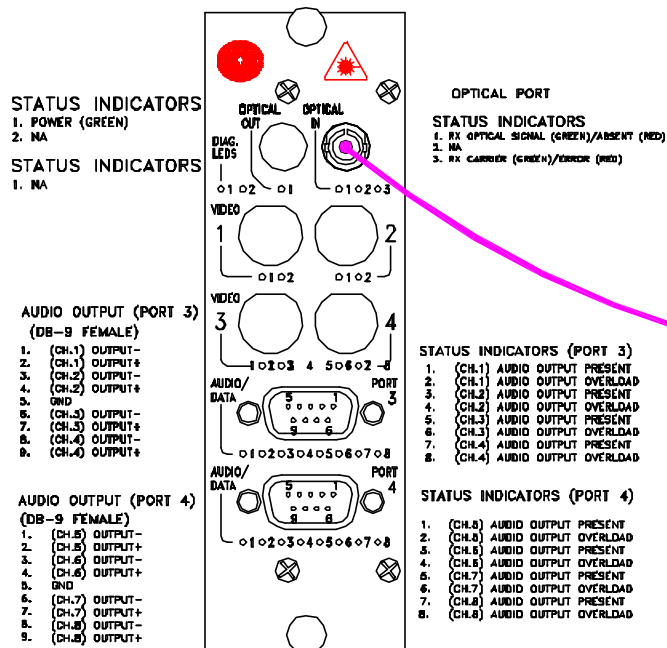
DR-8A- PINOUT DIAGRAM
