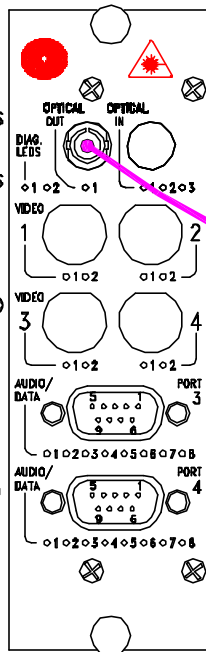
DT-8A-0 PINOUT DIAGRAM
