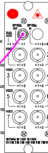
DT-8V-1 PINOUT DIAGRAM
