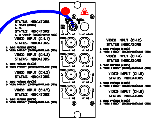
DT-8V-7 PINOUT DIAGRAM
