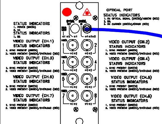
DR-8V-3 PINOUT DIAGRAM
