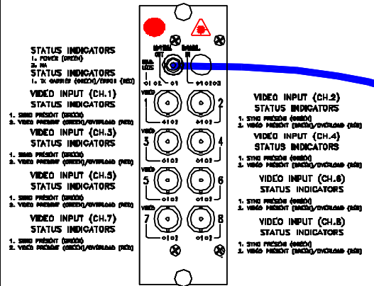
DT-8V-6 PINOUT DIAGRAM
