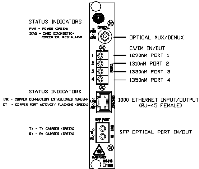
CD-1RE-20 PINOUT DIAGRAM
