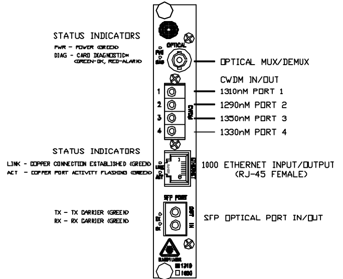
CM-1RE-20 PINOUT DIAGRAM
