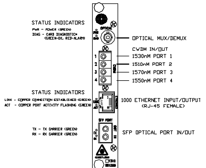
CM-1RE-21 PINOUT DIAGRAM
