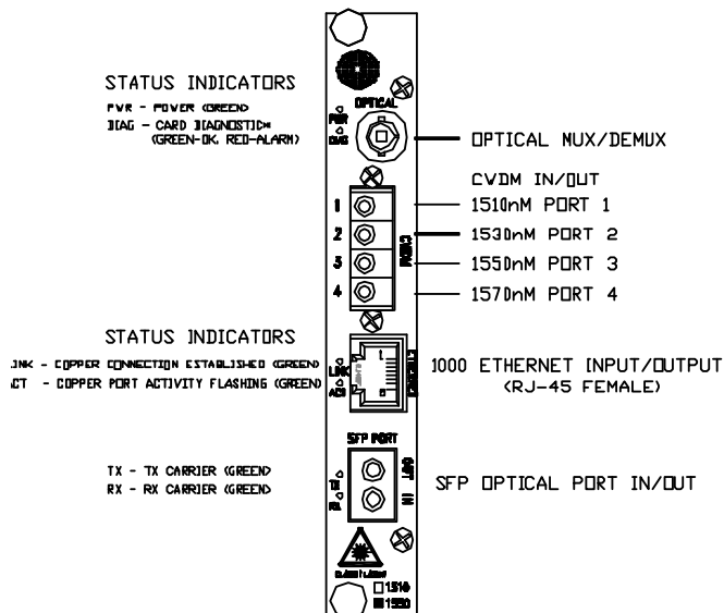
CD-1RE-21 PINOUT DIAGRAM
