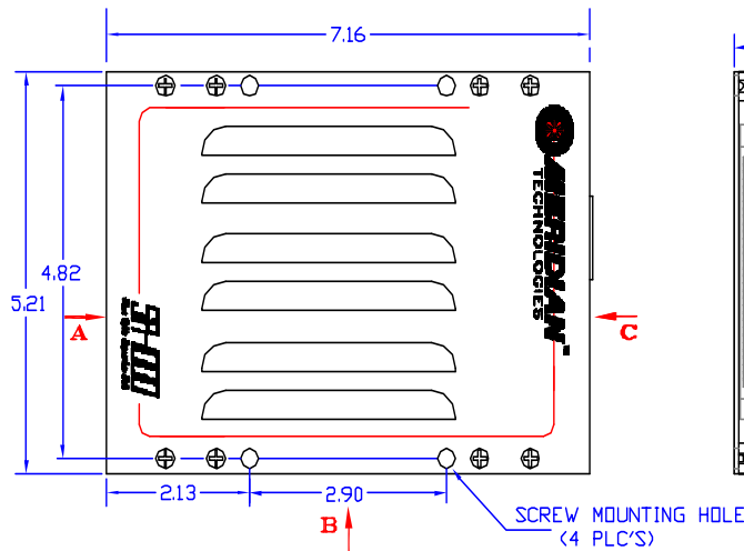
FRONT VIEW CARD ENTRY VIEW A
