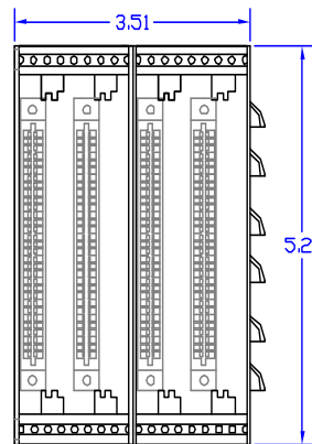
FRONT VIEW CARD ENTRY VIEW A
