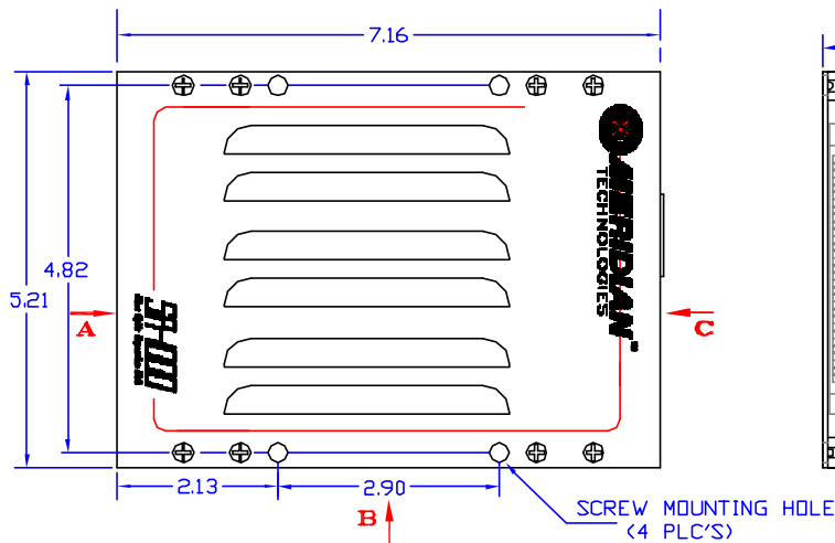
FRONT VIEW CARD ENTRY VIEW A
