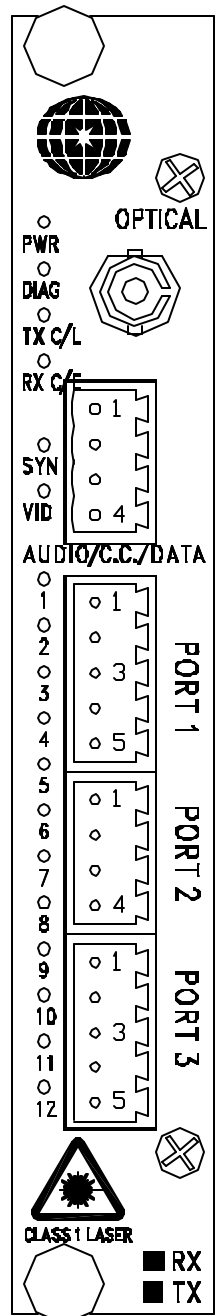
Figure 4.2 SXA/SXB-2C/2C-x-E63 1-Slot Module Front Panel Diagram
