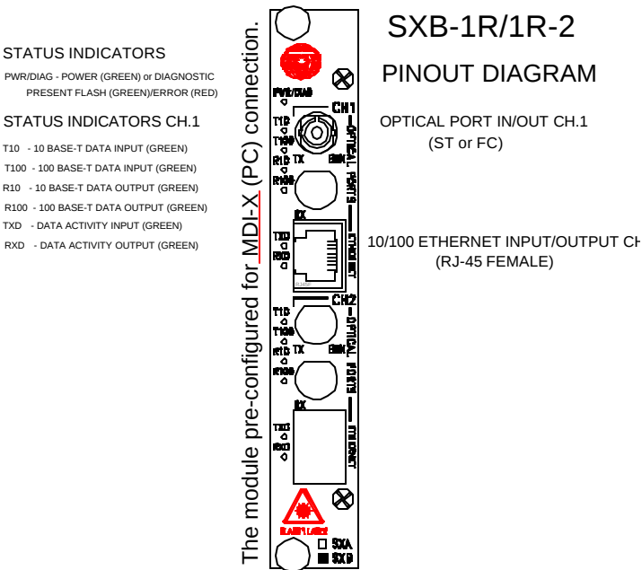
Figure 5.1 10/100 Ethernet Module Front Panel
