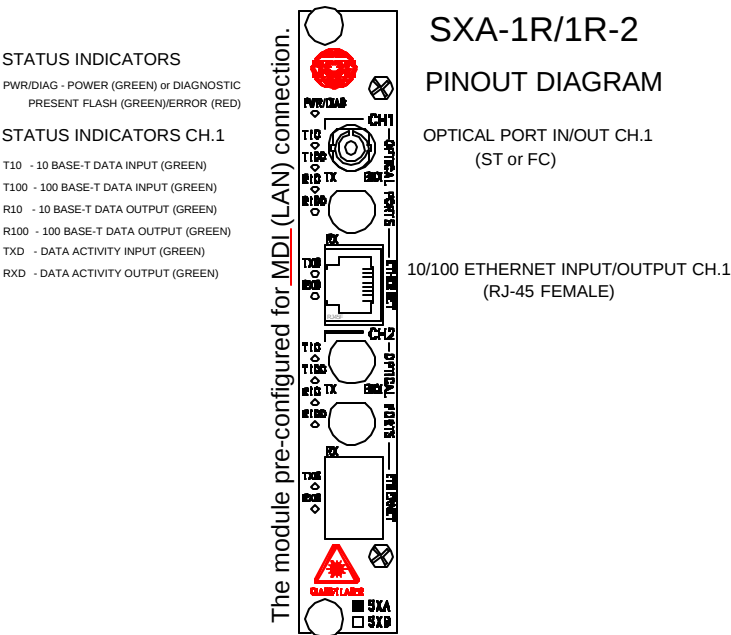
Figure 5.1 10/100 Ethernet Module Front Panel
