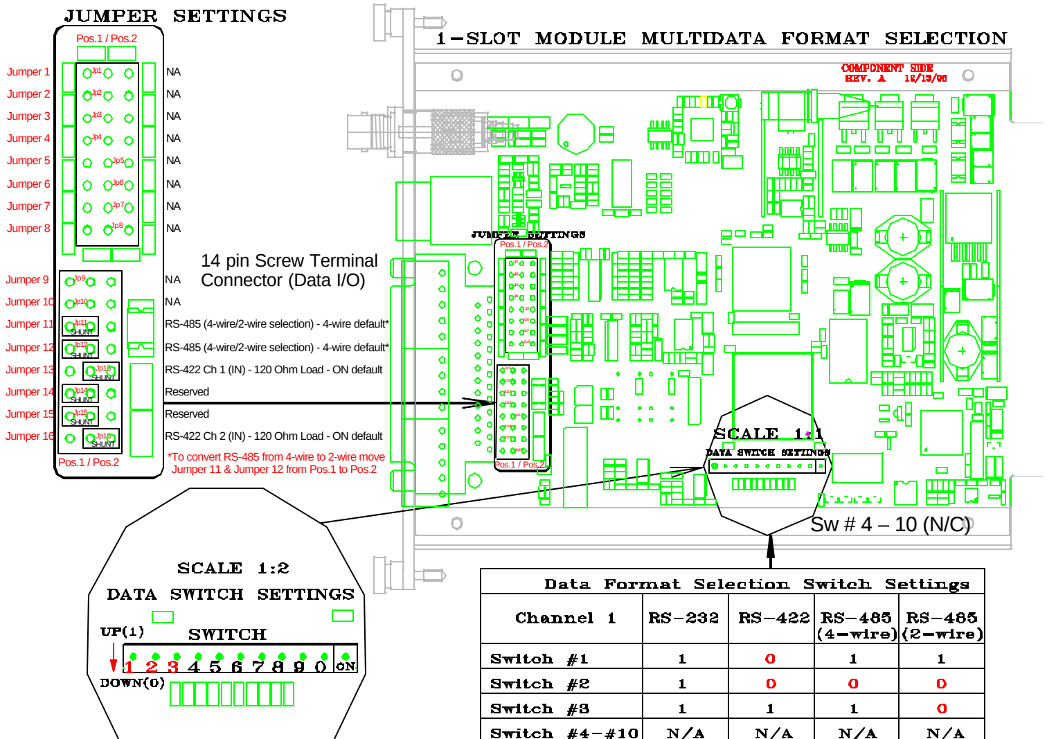
1-Slot Module Data Format Selection Switch
