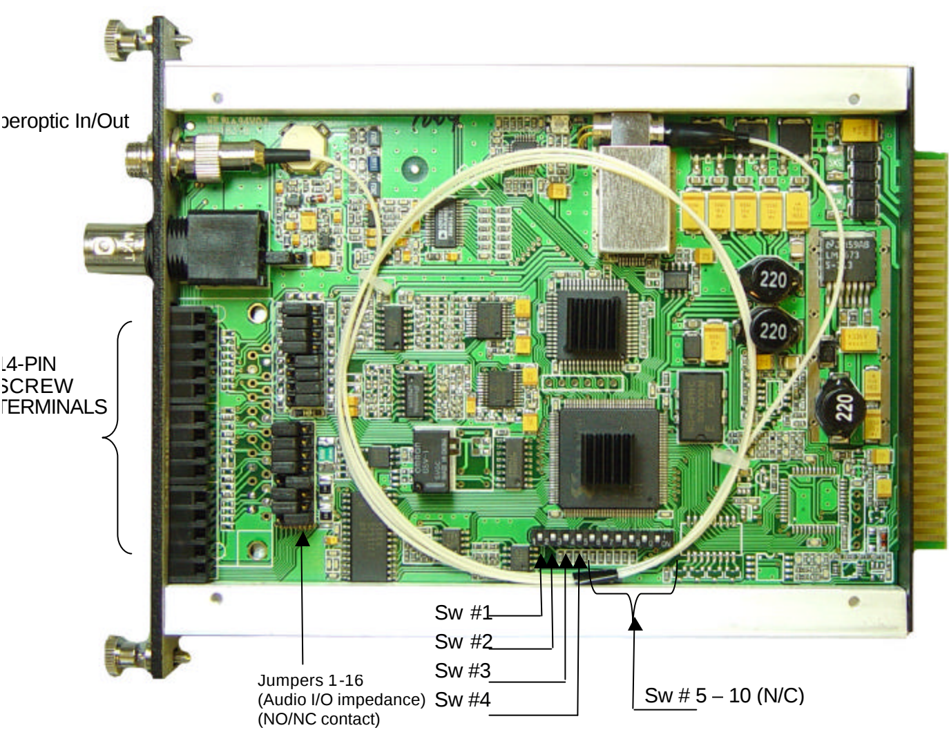
1-Slot Module Data Format Selection Switch & Jumper Location
