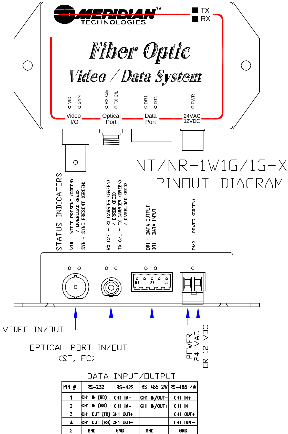
Figure 5.1 NT/NR-1W1G-1G-x Front Layout Diagram
