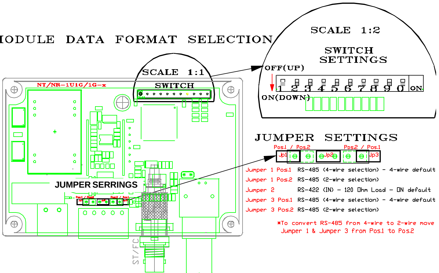
Figure 6.1 Module Switch and Jumper Location
