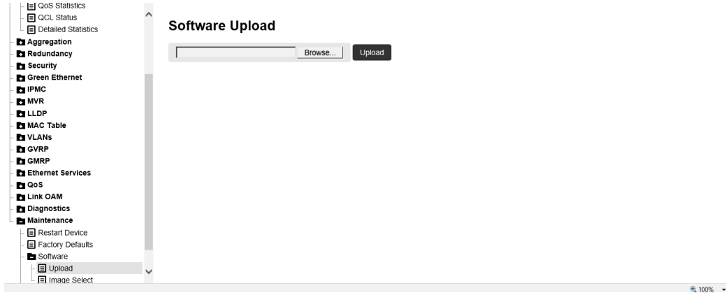
Update Firmware interface
