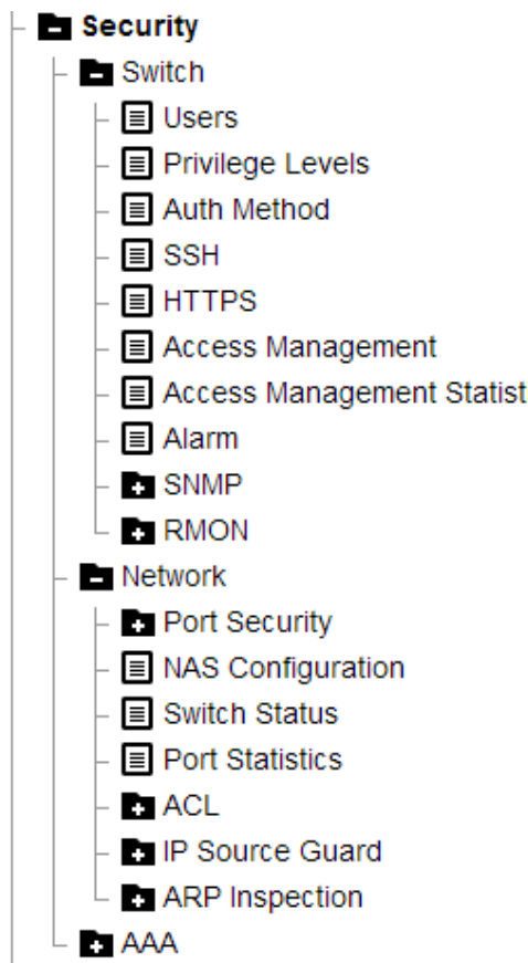
Menu navigation window interface
