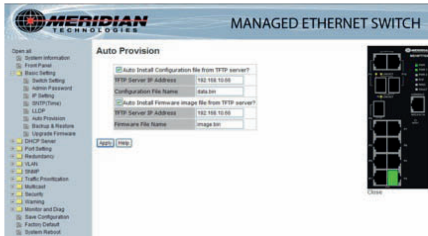
Auto Provision interface
