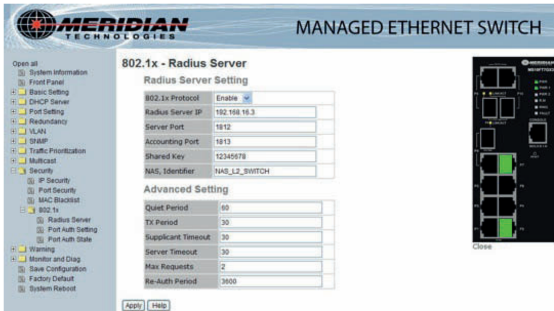
802.1x Radius Server interface
