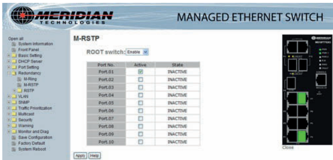
M-RSTP interface
