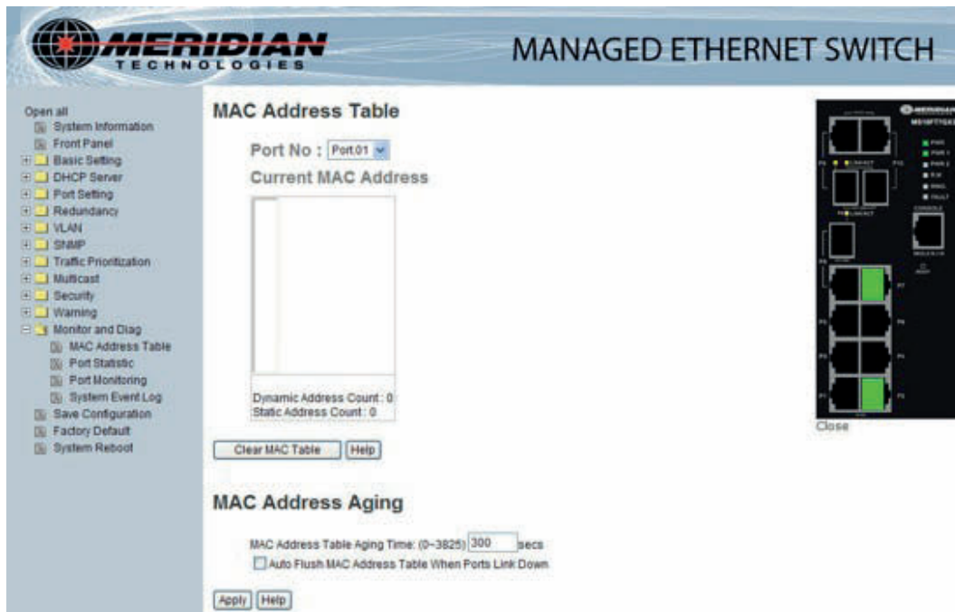
MAC Address Aging interface
