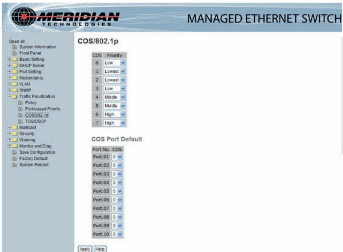
COS/802.1p interface
