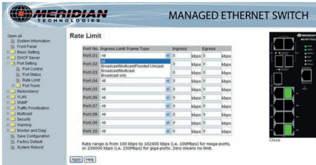
Rate Limit interface
