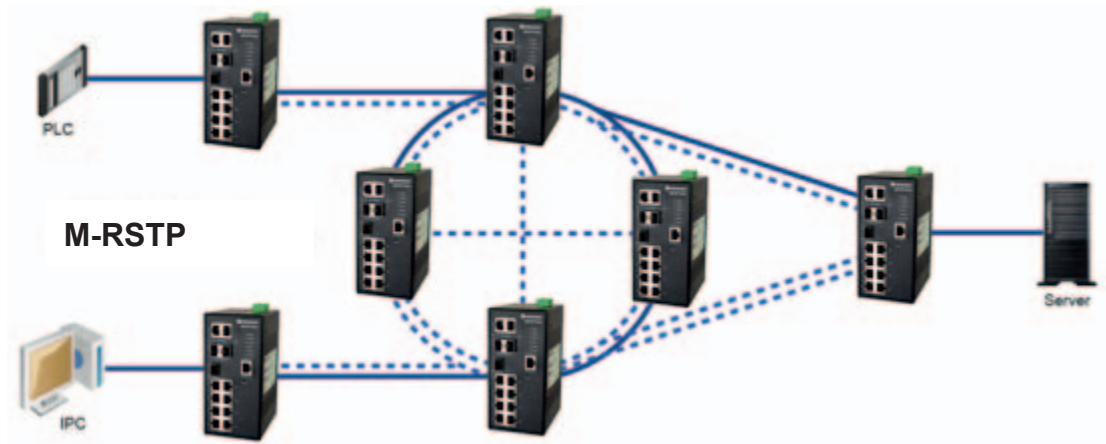
M-RSTP connection
