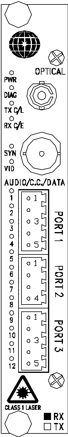
Figure 4.2 FR-1U1G/1G-x Front Panel Layout Diagram
