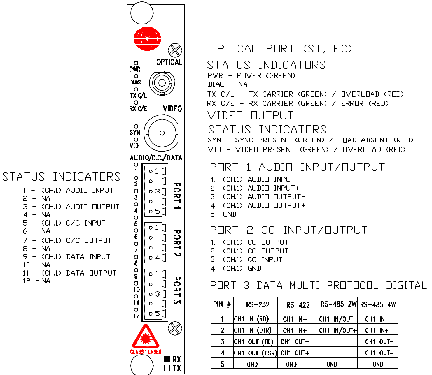
Figure 4.2 FR-1U1A1C1G-1A1C1G-x Front Pane Layout Diagram
