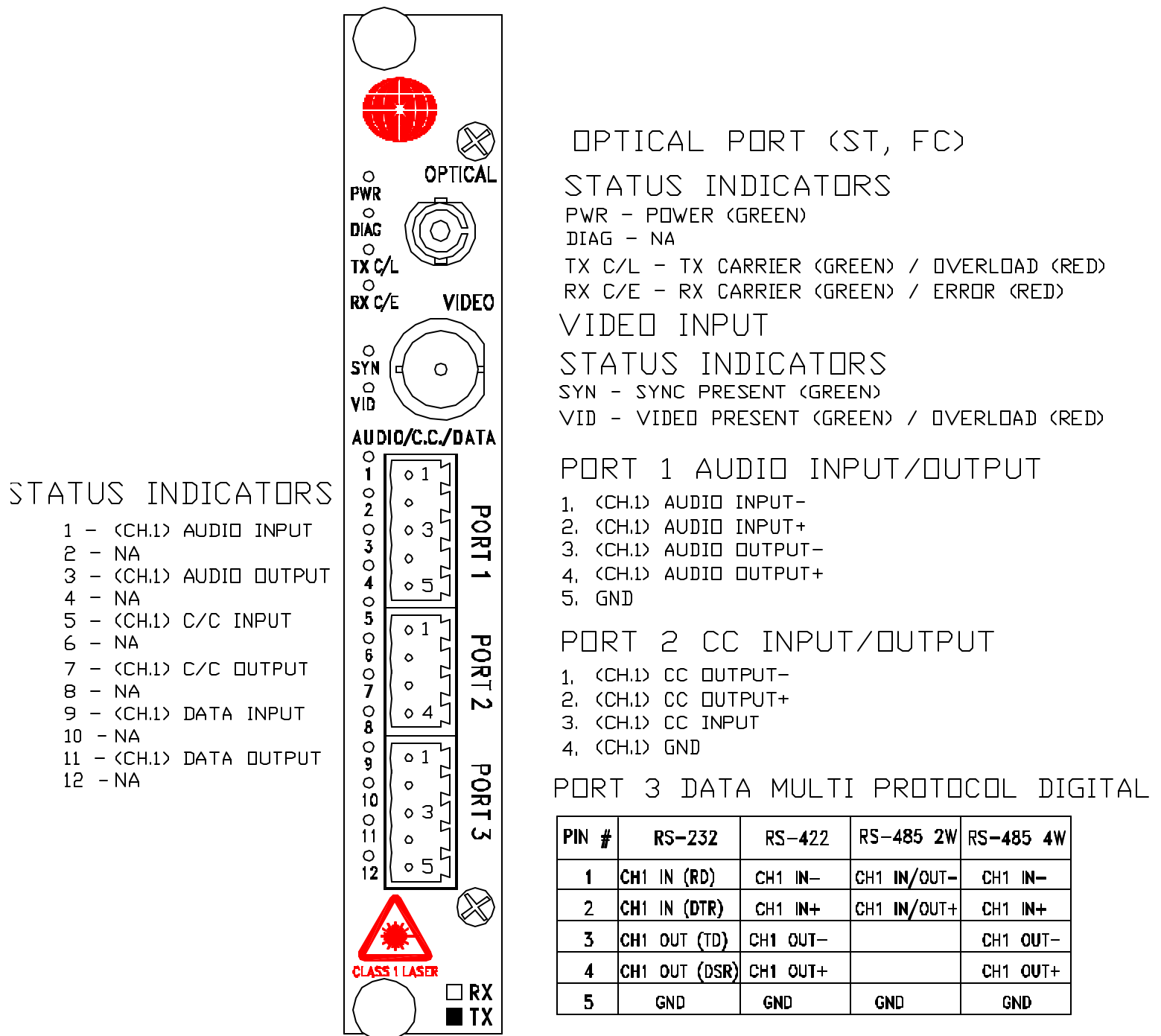
Figure 4.1 FT-1U1A1C1G-1A1C1G-x Front Pane Layout Diagram
