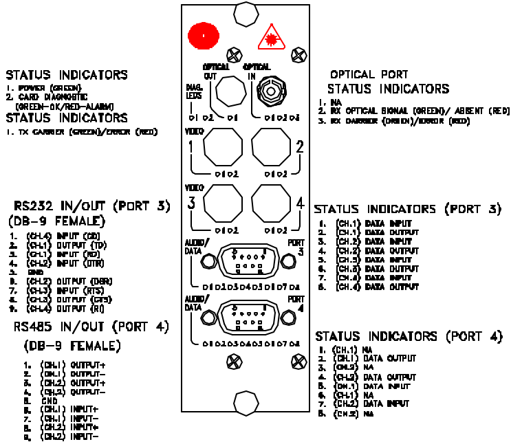
DXA-4D2K/4D2K-X PINOUT DIAGRAM
