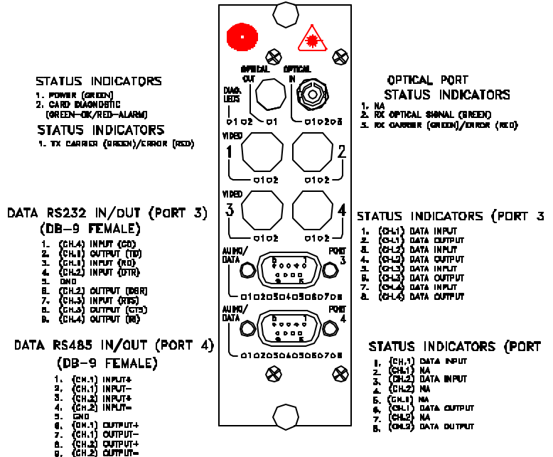
DXB-4D2K/4D2K-X PINOUT DIAGRAM
