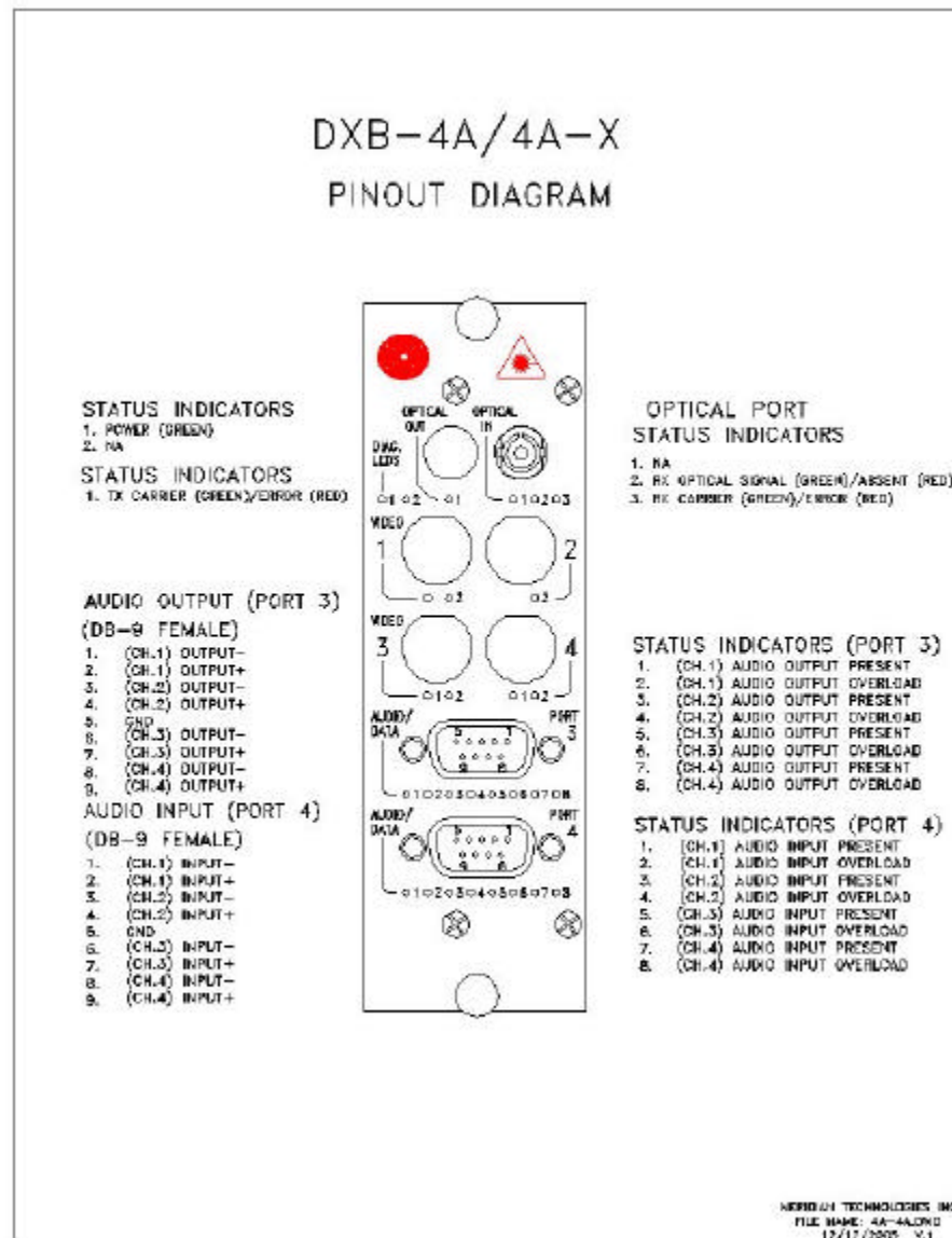
Figure 5.1 DXB-4A/4A-X Front Panel Layout/Pinout Diagrams
