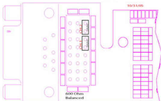
Audio jumper settings for 600Ohm Balanced Input/Output
