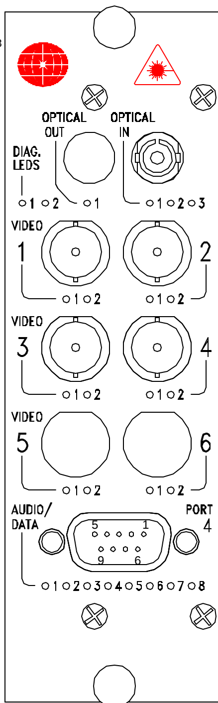
Figure 5.1 DT-4V(W)1F/1F Front Panel Pinout Diagram
