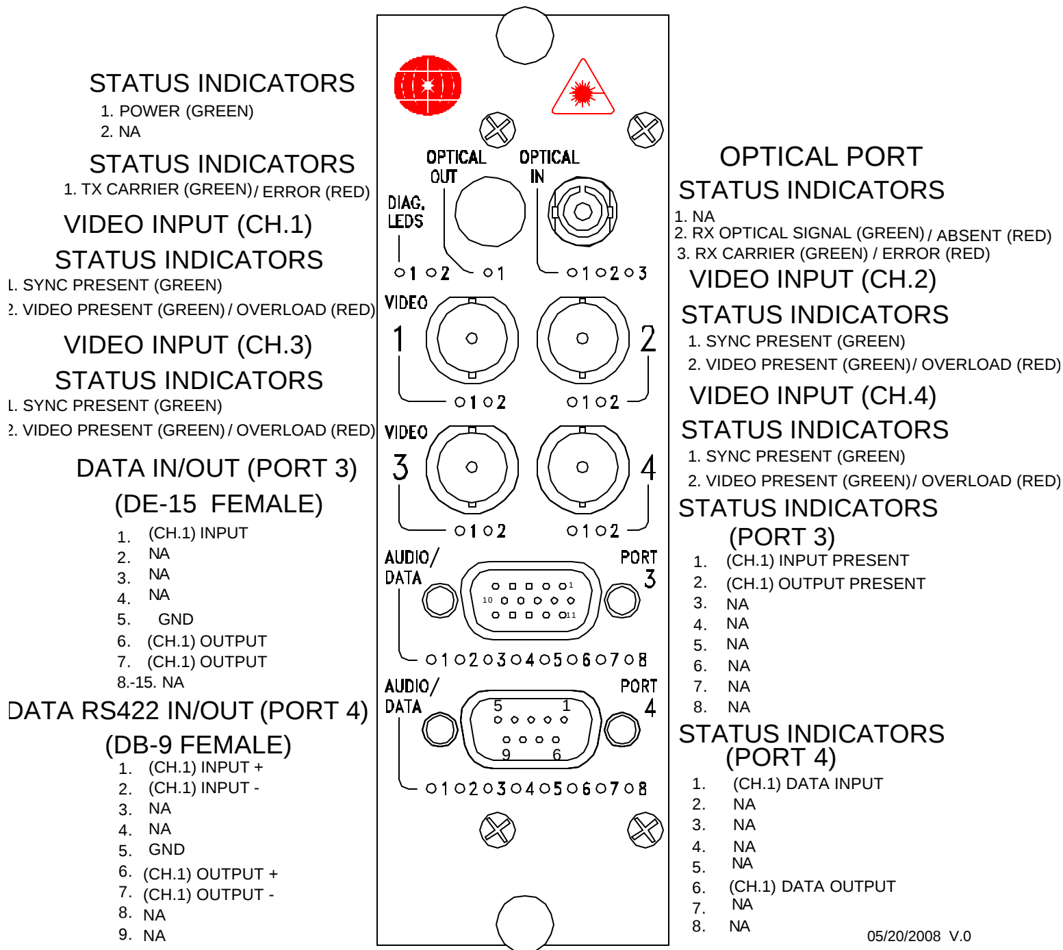
Figure 6.1 DT-4V(W)1C1F/1C1F-x Front Panel Layout Diagram
