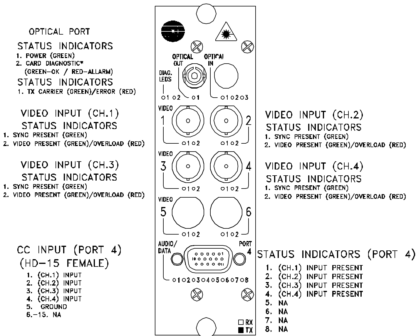
Figure 5.1 DT-4V(W)4C-x Module Front Panel Diagram.
