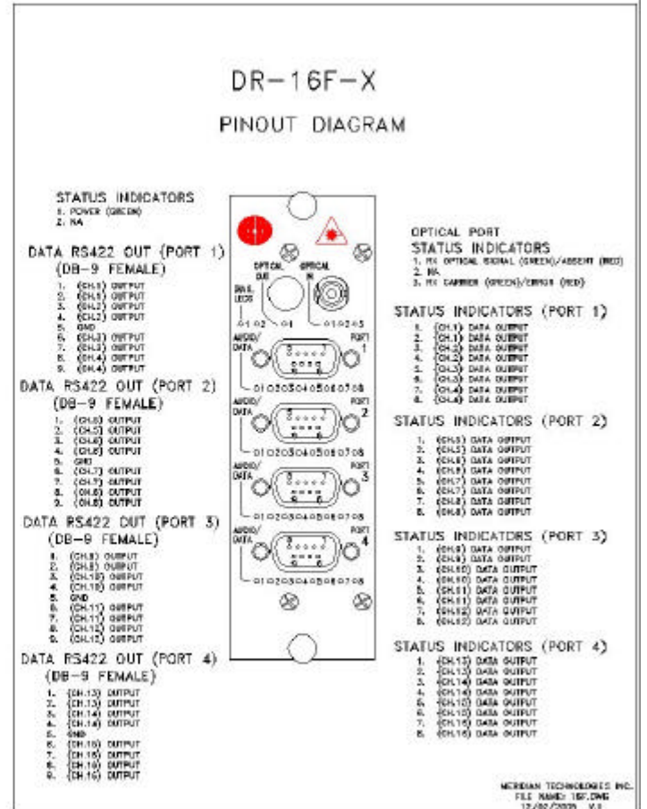
Figure 4.1 Front Panel Layout/Pinout Diagrams
