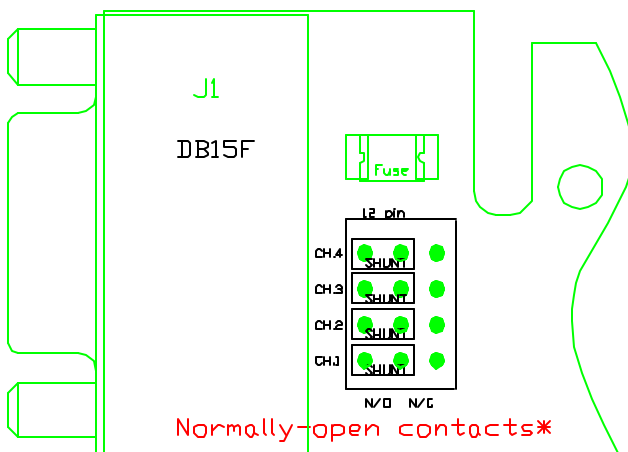
Jumper Setting For Contact Closure BI-DI
