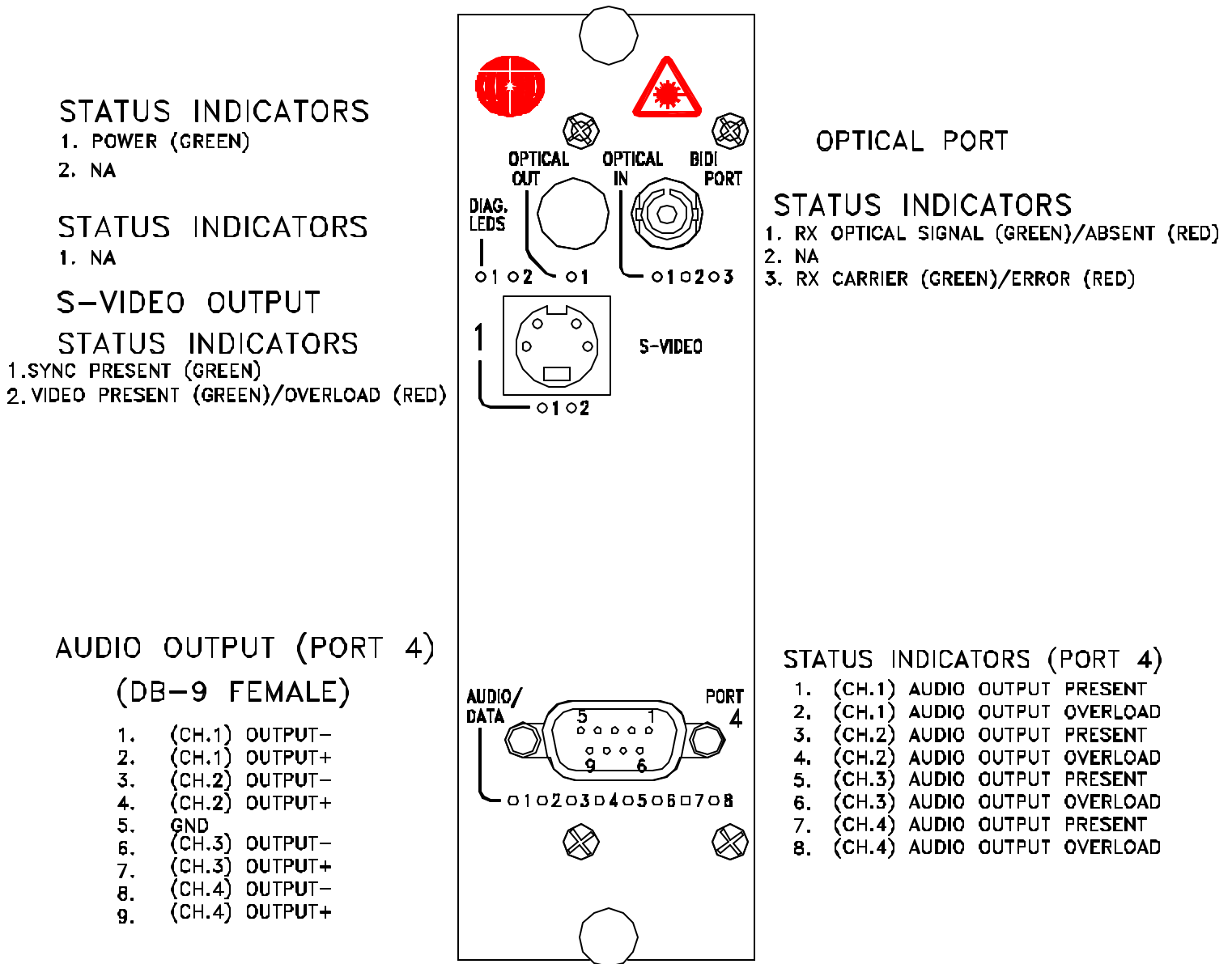
Figure 7.2 DR-1S4A-x Front Panel Diagram
